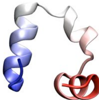
villin headpiece 3 months on 329 CPUs
