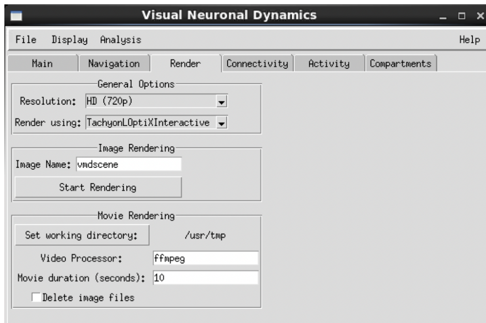
Figure 11: VND window with 'Render' tab. The options define OpenGL resolution and render selection to generate high quality images.
