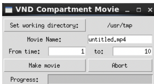
Figure 12: Example of the VND movie control window for the compartment data animation. The user can define the working directory, the root name of the files generated, the animation interval, and also monitor the progress of the rendering.
