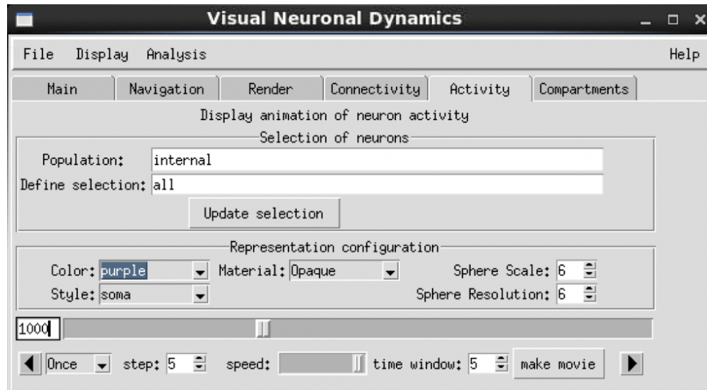
Figure 7: VND window with 'Activity' tab. Menus define selection of neurons for spike activity (e.g. 'all'), configuration (e.g. color 'purple', style 'soma') and animation playback (e.g. step '5', time window '5').
