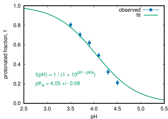
Figure 4: Collecting the protonated fraction observed at each pH value constitutes a titration curve (shown here for aspartate dipeptide). A pK_a value can be extracted by fitting to the Henderson-Hasselbalch equation. Error bars represent estimated 95% confidence intervals.
