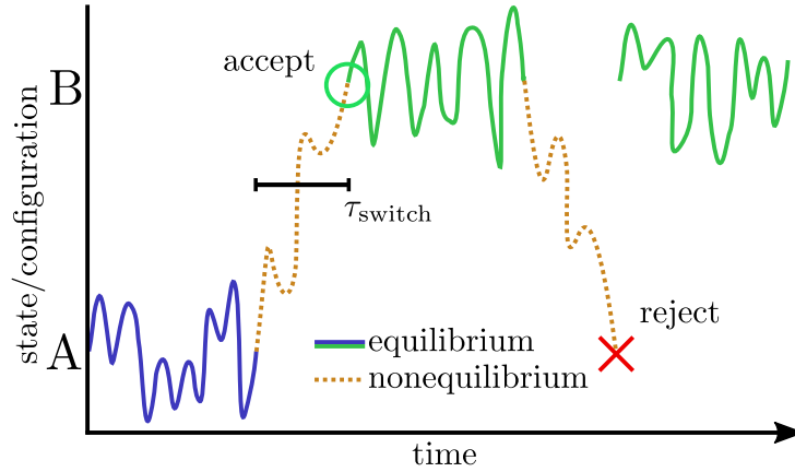
Figure 2: The basic constant-pH MD scheme in NAMD is to alternate equilibrium sampling in a fixed protonation state followed by a neMD/MC move to sample other protonation states. The latter move can be accepted or rejected. If accepted, the simulation continues in the new protonation state. If the move is rejected, sampling continues as if the move were never attempted at all.
