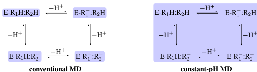
Figure 1: The core difference between conventional and constant-pH MD can be illustrated by a simple enzyme E with four protonation states describing the occupancy of two titratable residues, R_1 and R_2 . A conventional MD simulation handles the states separately (left panel). The relative importance of the states must be known beforehand or computed by other means. Conversely, a constant-pH MD simulation handles the states collectively and actively simulates interconversion (right panel). Determining the relative importance of the states is a direct result of the simulation.
