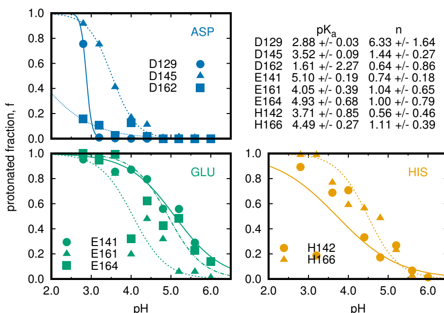
Figure 6: Titration curves can be computed for BBL using the cphanalyze program and a simple counting procedure. Note that many irregularities in sampling at different pH values are somewhat hidden by the reweighting algorithm used in figure 5. All titratable residues that actively changed in the selected pH range have been sorted by type and their macroscopic titration curves were fit to the Hill equation. Error bars represent estimated 95% confidence intervals.
