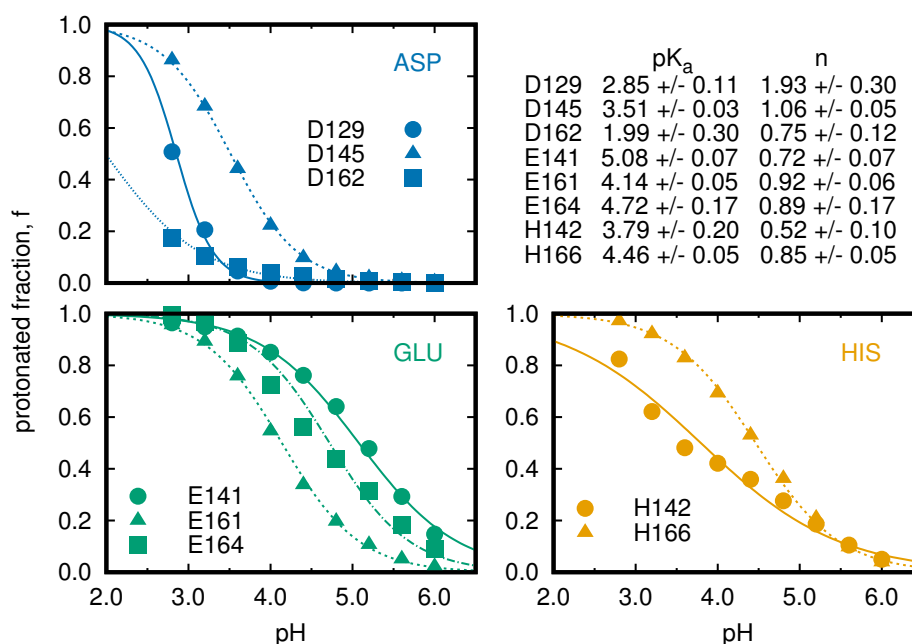
Figure 5: Titration curves can be computed for BBL using the cphanalyze program and a specialized reweighting procedure [1]. All titratable residues that actively changed in the selected pH range have been sorted by type and their macroscopic titration curves were fit to the Hill equation. Error bars represent estimated 95% confidence intervals.
