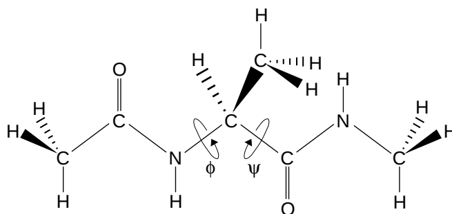
Figure 6: Blocked N -acetyl- N' -methyl-L-alanylamide (NANMA), featuring torsional angles \varphi and \psi
