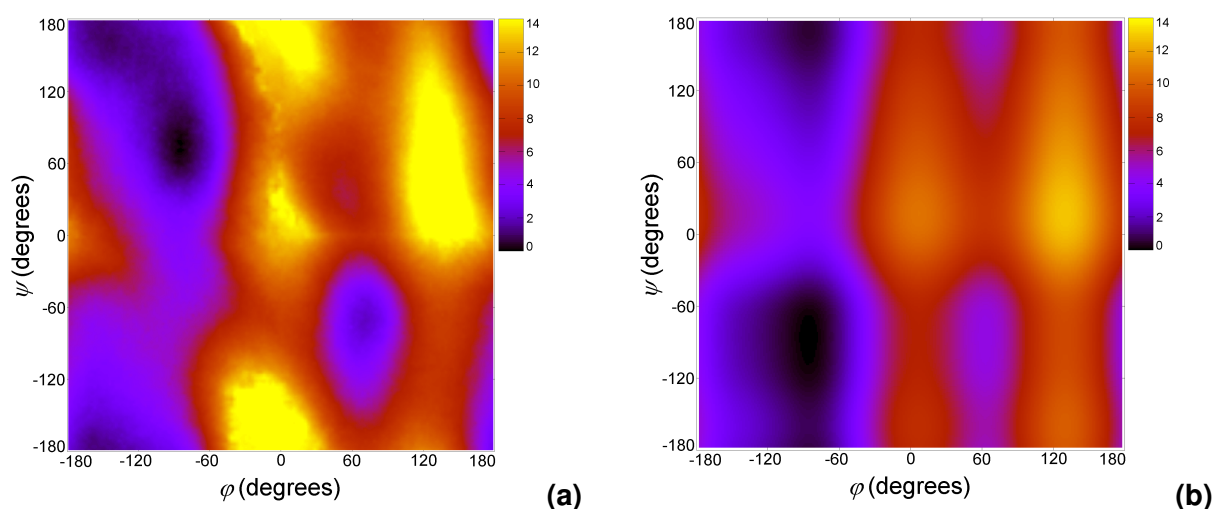
Figure 7: Free-energy surface characterizing the conformational equilibrium of N-acetyl-N'-methylalaninamide in the gas phase (a) and in bulk water (b), derived from a two-dimensional ABF simulation that uses the \varphi and \psi torsional angles as the reaction coordinate.
