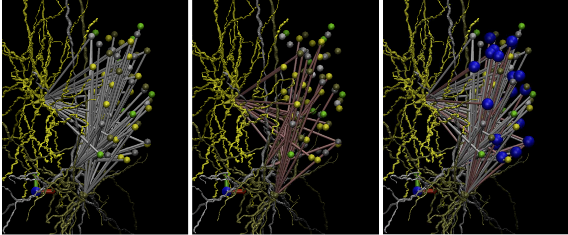
Figure 9: VND OpenGL window showing 300_cell example model with drawn edges. Connection representations: (left) source 'stride 100', target '(soma x > 0) && (soma y > 0)', coloring method 'white', style 'simple_edge'. (middle) source '(soma x > 0) && (soma y > 0)', target 'stride 100', coloring method 'pink', style 'simple_edge'. (right) All of the above and source '(soma x > 0) && (soma y > 0)', target 'stride 100', coloring method 'blue', style 'source_soma' and 'Sphere Scale' 5. All representations have material 'Opaque'.
