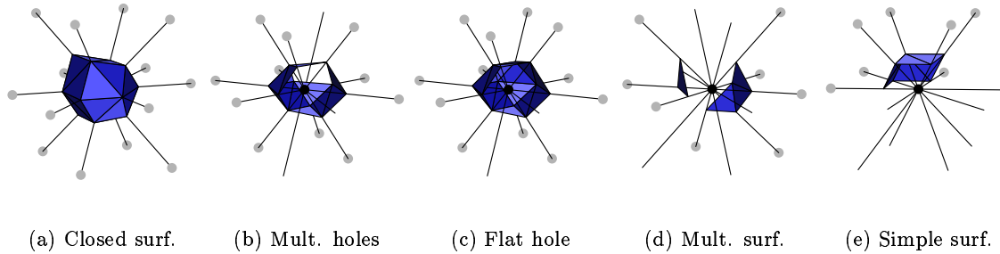
Figure 5: Topology preservation. (a) to (e) show the possible topological cases considered during vertex clustering. (a), (b) and (c) cannot be clustered. (d) and (e) can be, with one new vertex per surface. Clustering of the vertices in (c) might lead to non-manifold surfaces.
