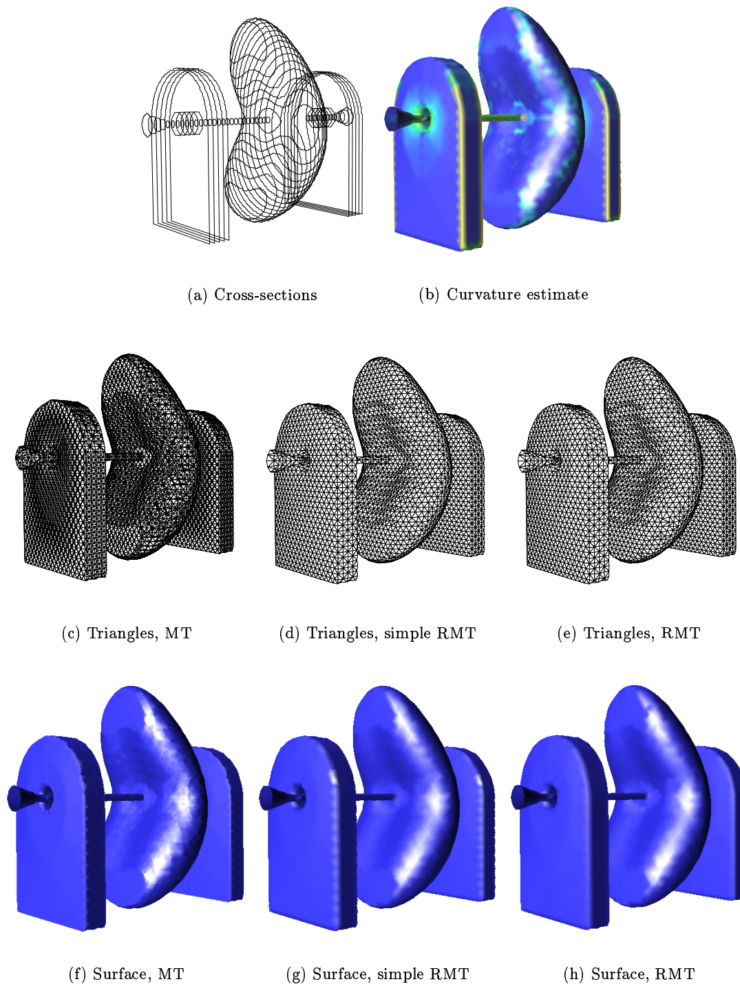
Figure 7: Example iso-surface. (a) shows the object cross-sections from which the distance function was derived. (c) and (f) show the result of using MT, (d) and (g) include vertex clustering, and (e) and (h) also include weighting of the vertex position using curvature. (b) shows the curvature estimate mapped to colours — blue indicates low curvature through green then red indicating high curvature.
