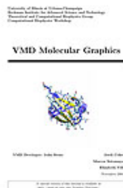
Figure 10: VMD Molecular Graphics Title Page
