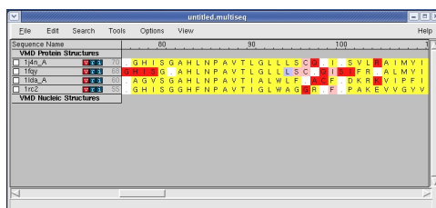
Figure 19: View of the Residue Selection for Q \geq 0.5 in the Sequence Display window.
