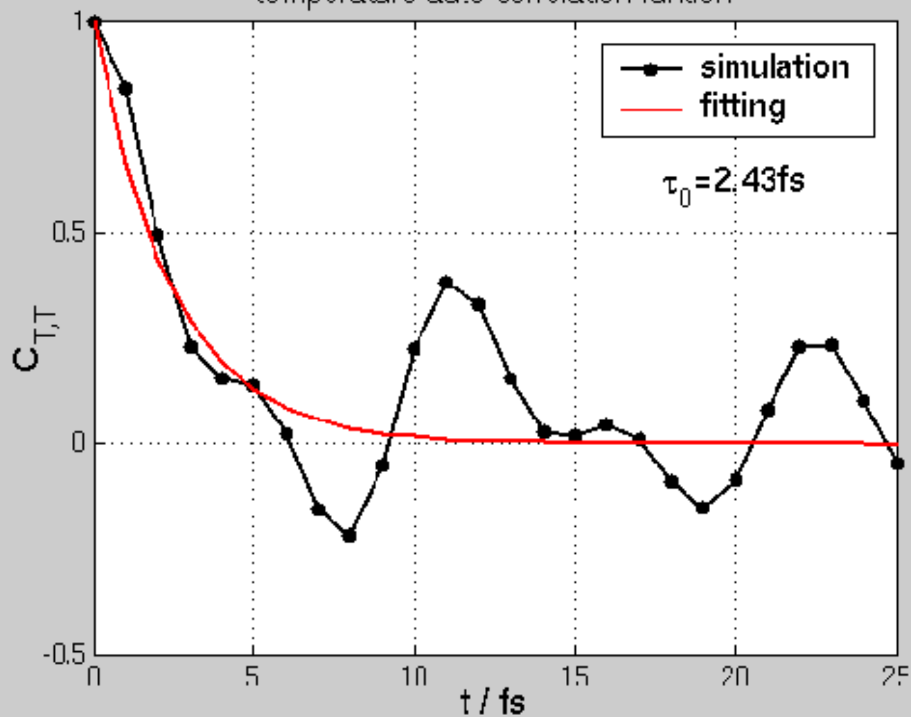
temperature auto-correlation function
