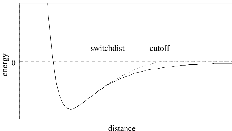
Figure 1: Graph of van der Waals potential with and without the application of the switching function. With the switching function active, the potential is smoothly reduced to 0 at the cutoff distance. Without the switching function, there is a discontinuity where the potential is truncated.
