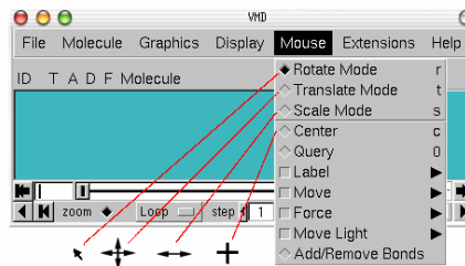
Figure 3: Mouse modes.
