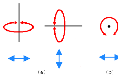
Figure 2: Rotation modes.
