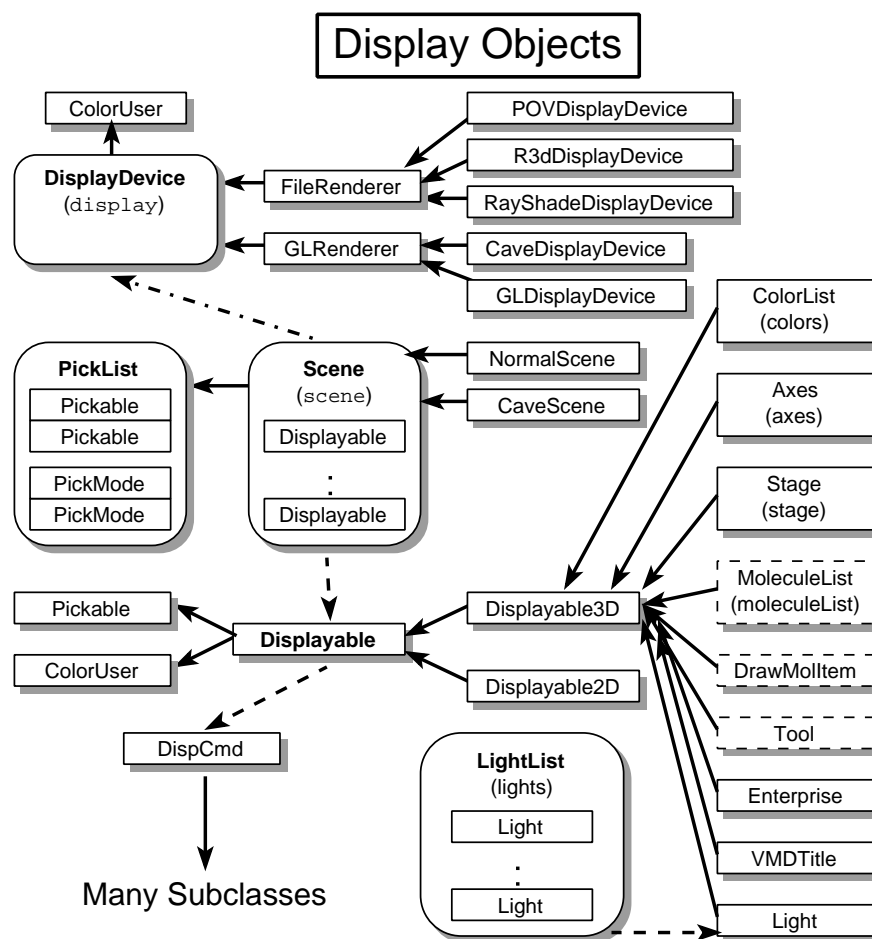
Figure 5.2: Display objects used in VMD.
