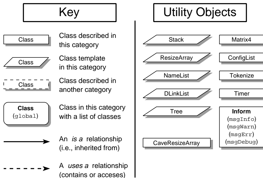
Figure 5.1: Utility objects used in VMD, and a key describing the function of diagrammatic items in these object description figures.
