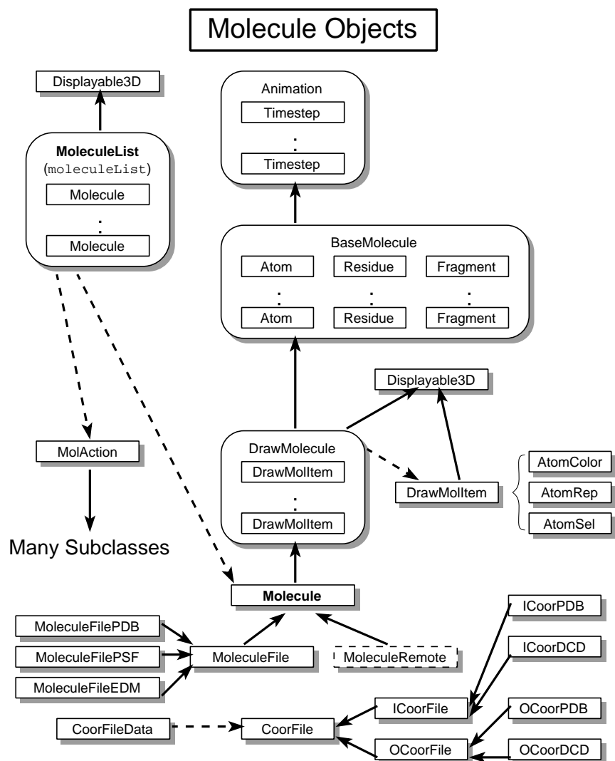
Figure 5.3: Molecule objects used in VMD.
