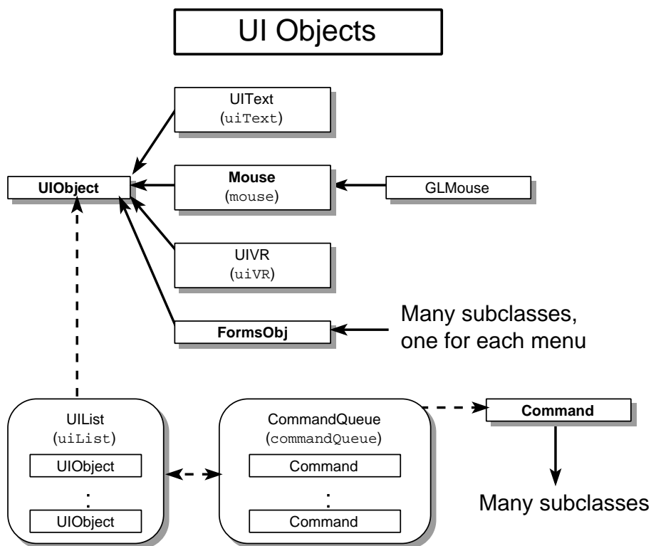
Figure 5.5: User interface objects used in VMD.
